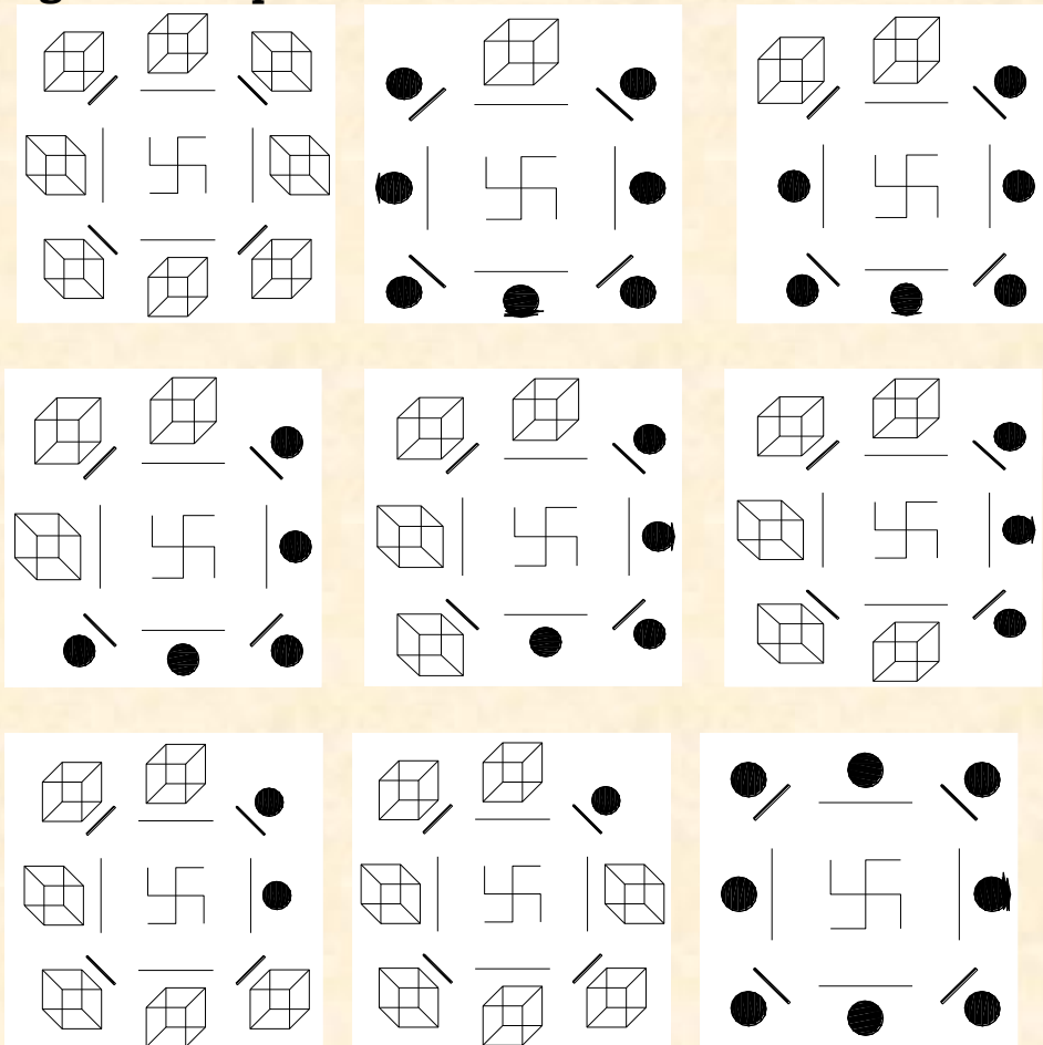
Figure of 4-space
